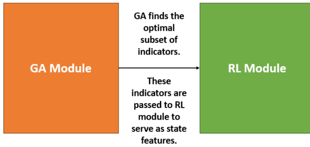
Fig. 8. Loosely coupled approach for state feature selection proposed by Hryshko et al. [81].
