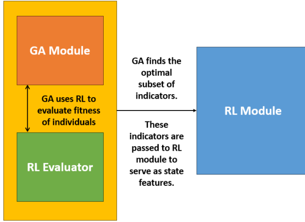
Fig. 7. Tightly coupled approach for state feature selection proposed by Dempster et al. [49].
