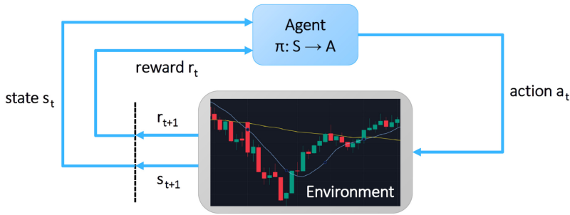
Fig. 4. Reinforcement learning framework (adapted from Sutton and Barto [173]).
